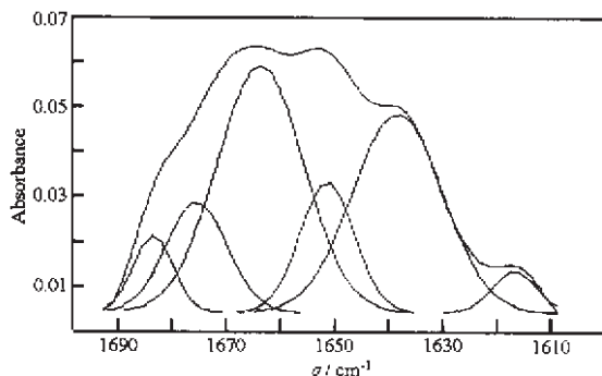
Fig. 3 Decomposition of the amide I band of \beta 2 in PBS buffer (D 2 O) at 20 \text{ }^\circ\text{C}
