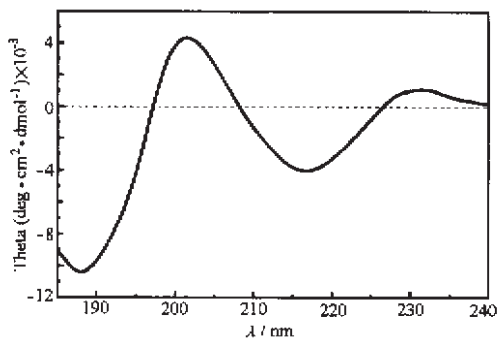
Fig. 2 The CD spectrum of \beta 2 in PBS buffer pH 7.04, 0.68 \text{ mmol} \cdot \text{L}^{-1} at 20 \text{ }^\circ\text{C}
